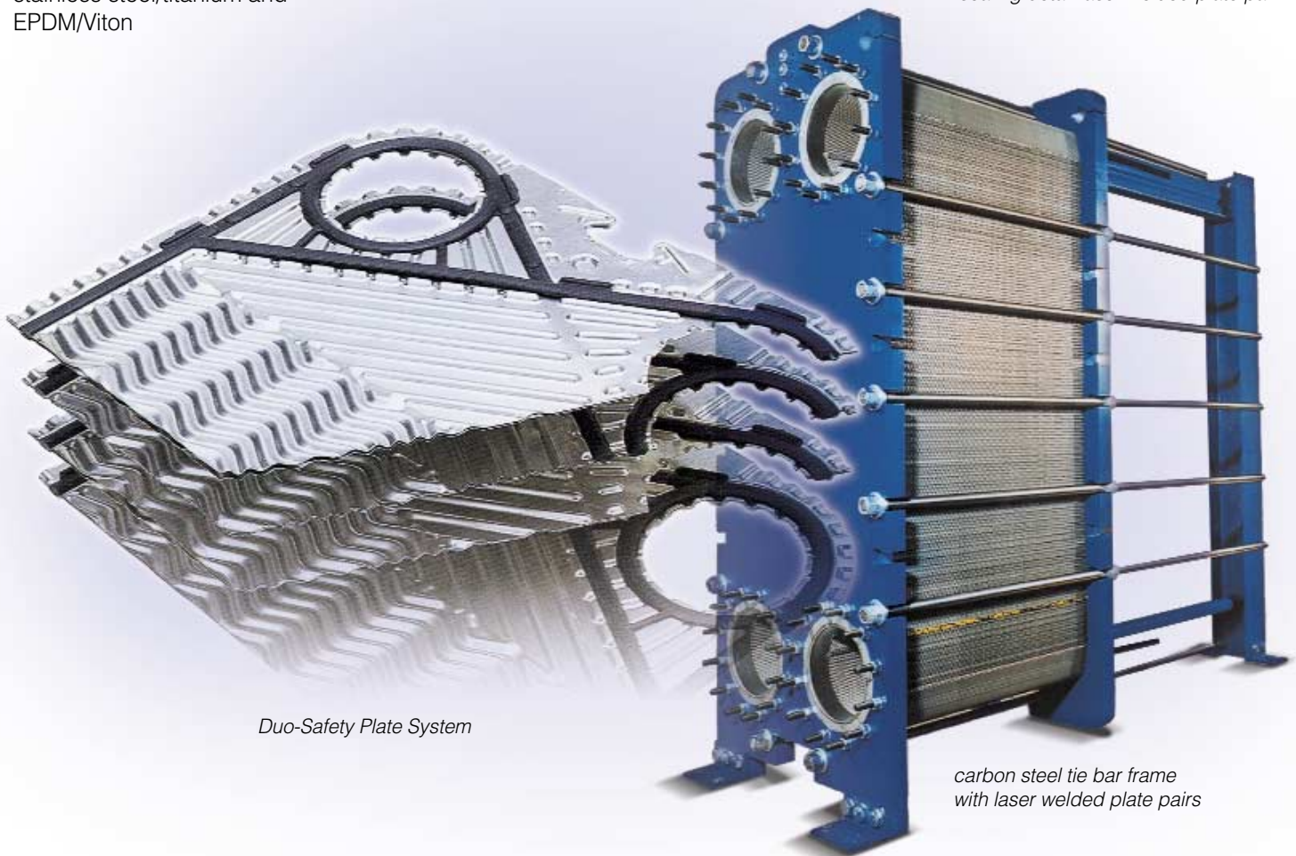
sealing detail laser welded plate pair
