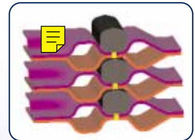
sealing detail laser welded plate pair
